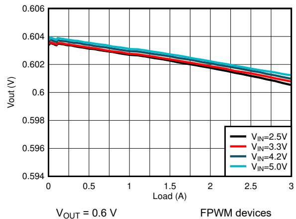
Figure 9-6. Load Regulation
