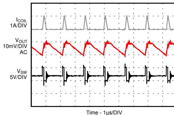
Figure 9-28. PSM Operation
