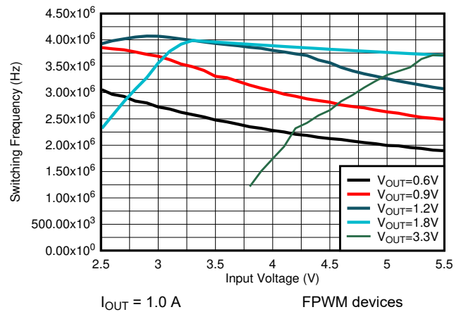
Figure 9-26. Switching Frequency
