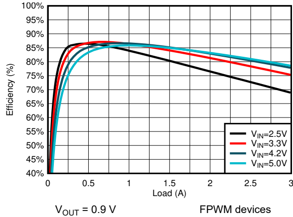
Figure 9-9. Efficiency
