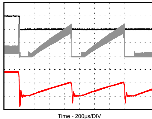
Figure 9-34. HICCUP Short Circuit Protection
