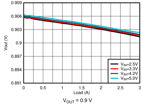
Figure 9-10. Load Regulation
