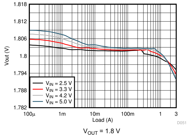
Figure 9-16. Load Regulation
