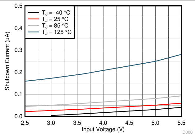
Figure 7-4. Shutdown Current
