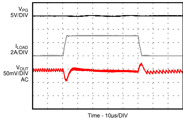
Figure 9-33. Load Transient
