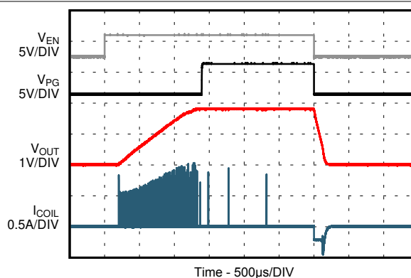
Figure 9-28. PSM Operation
