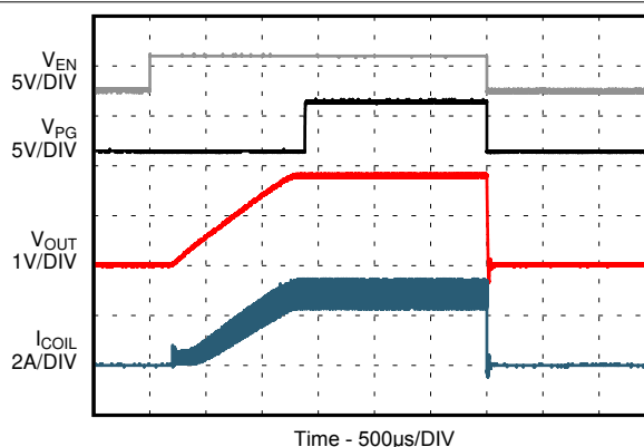
Figure 9-30. Start-Up with No-Load
