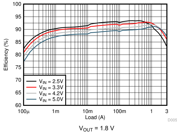
Figure 9-15. Efficiency
