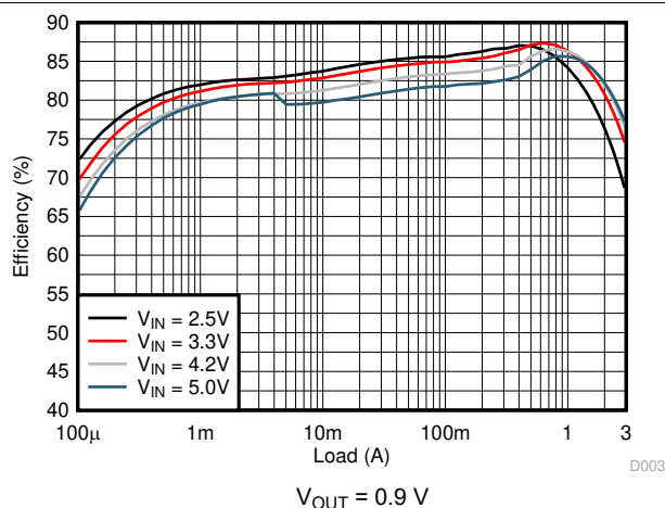
Figure 9-7. Efficiency
