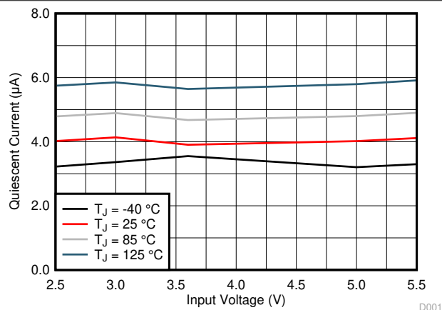
Figure 7-3. Quiescent Current
