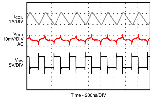
Figure 9-27. PWM Operation
