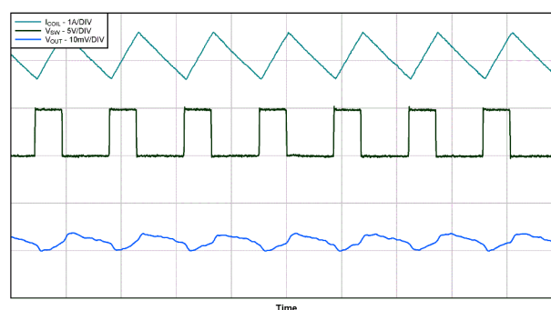
Figure 9-27. PWM Operation
