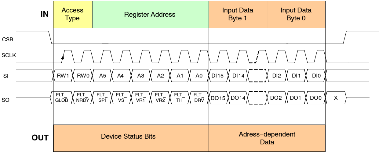
Figure 18. SPI Frame
