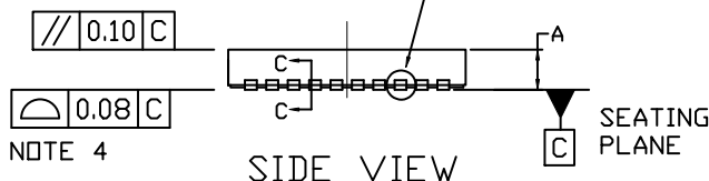
DETAIL B
