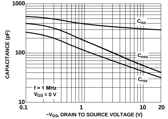
Figure 20. Capacitance vs. Drain to Source Voltage
